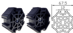
Polea 70 octogonal | 61.005.006
