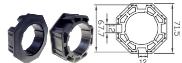
Corona 70 octogonal | 61.005.106
